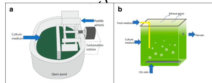
Figure 1. (a) Open raceway pond, (b) photobioreactor. Reprinted with the permission from [65]. Copyright 2022 Springer Nature.
