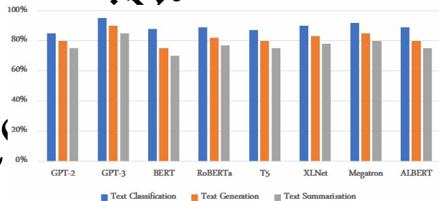
Figure 2. Performance comparison of language models on text classification, text generation, and text summarization tasks.
